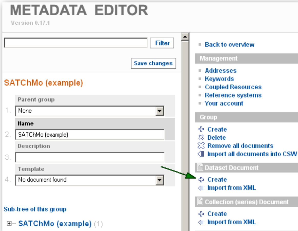
Figure 20: Creating dataset metadata document
